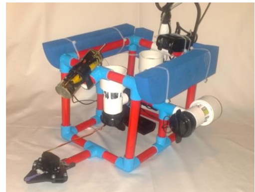
ROV design
